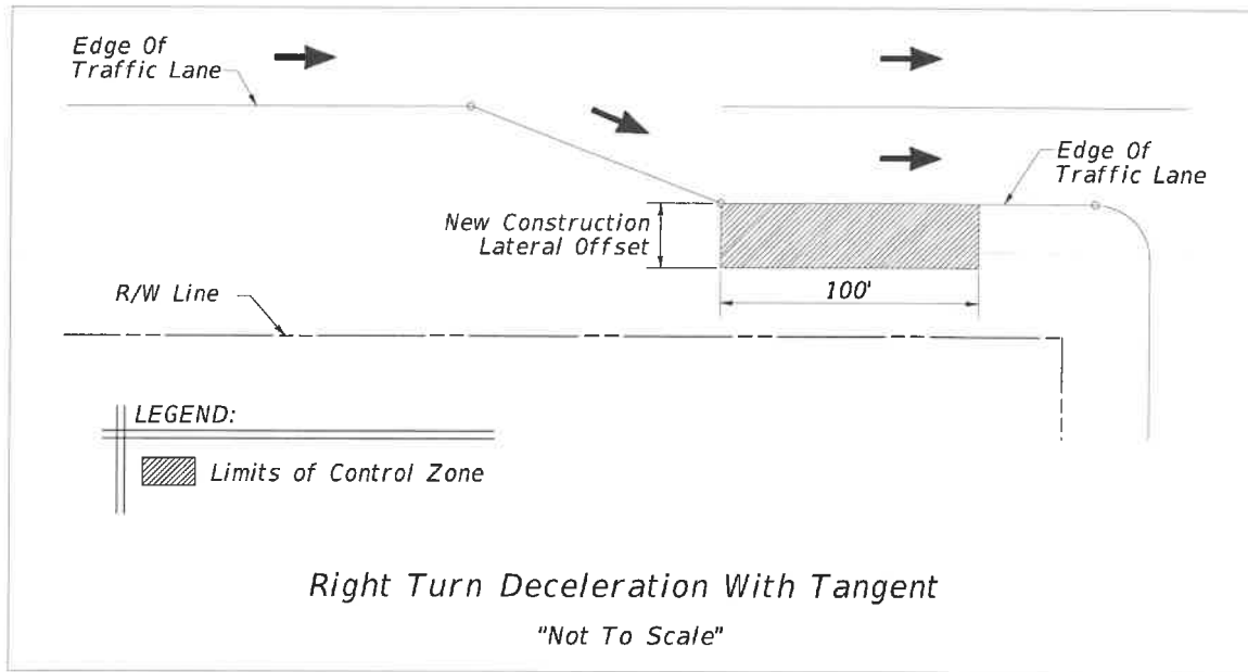
Figure 215.2.6 Right Turn Deceleration with Tangent
