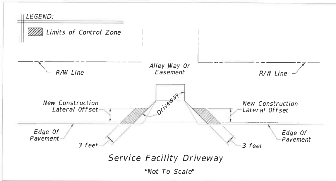
Figure 215.2.10 Service Facility Driveway
