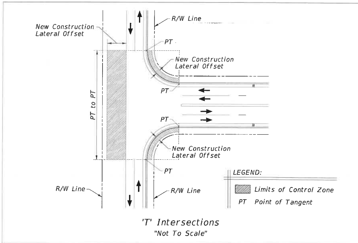
Figure 215.2.5 'T' Intersection
