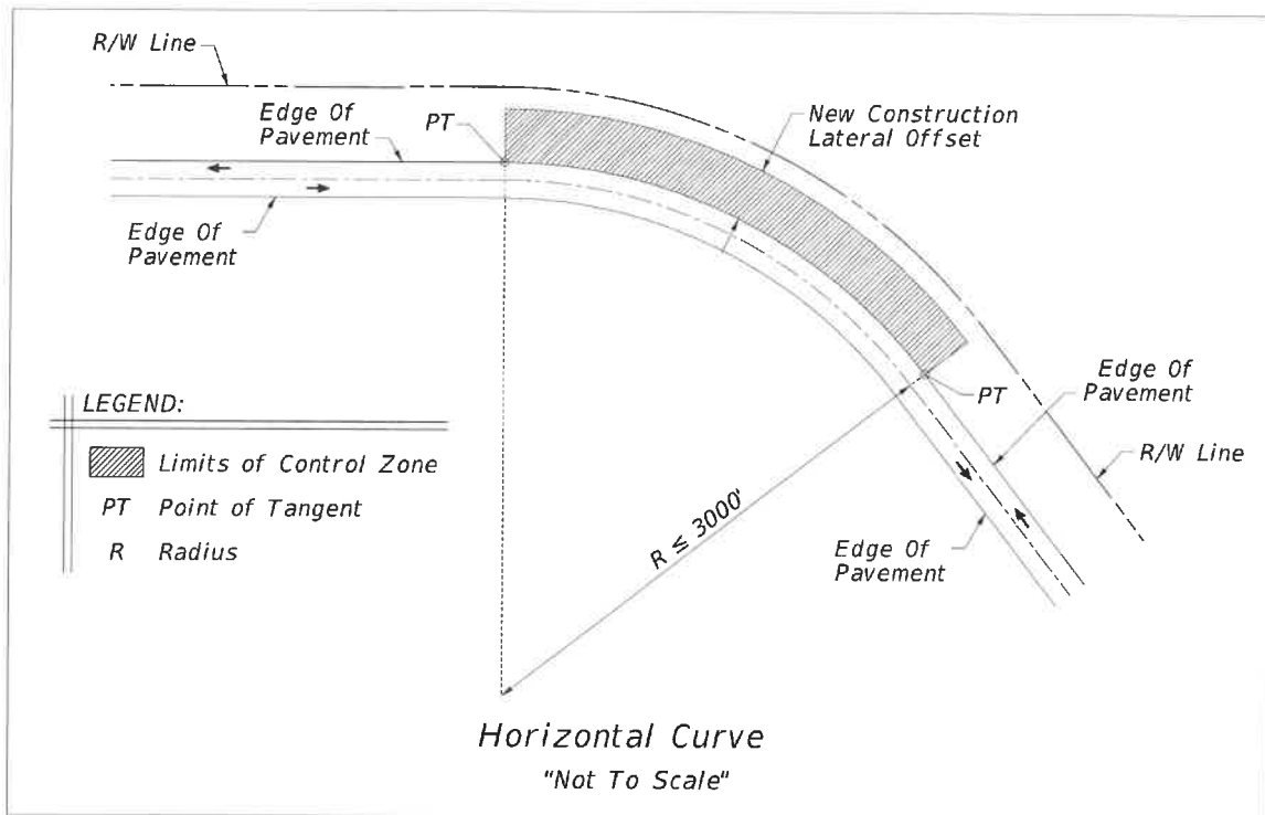
Figure 215.2.12 Horizontal Curve
