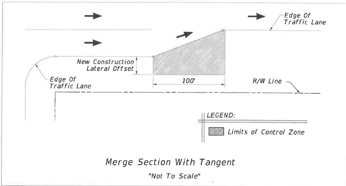
Figure 215.2.8 Merge Section with Tangent
