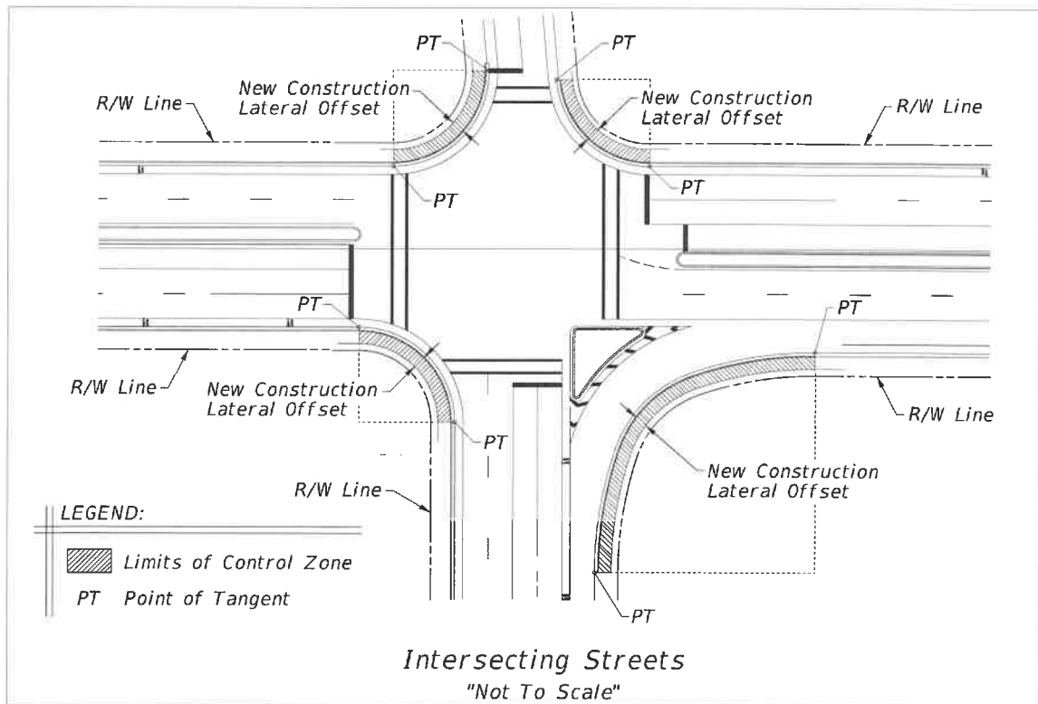
Figure 215.2.4 Intersection Radii
